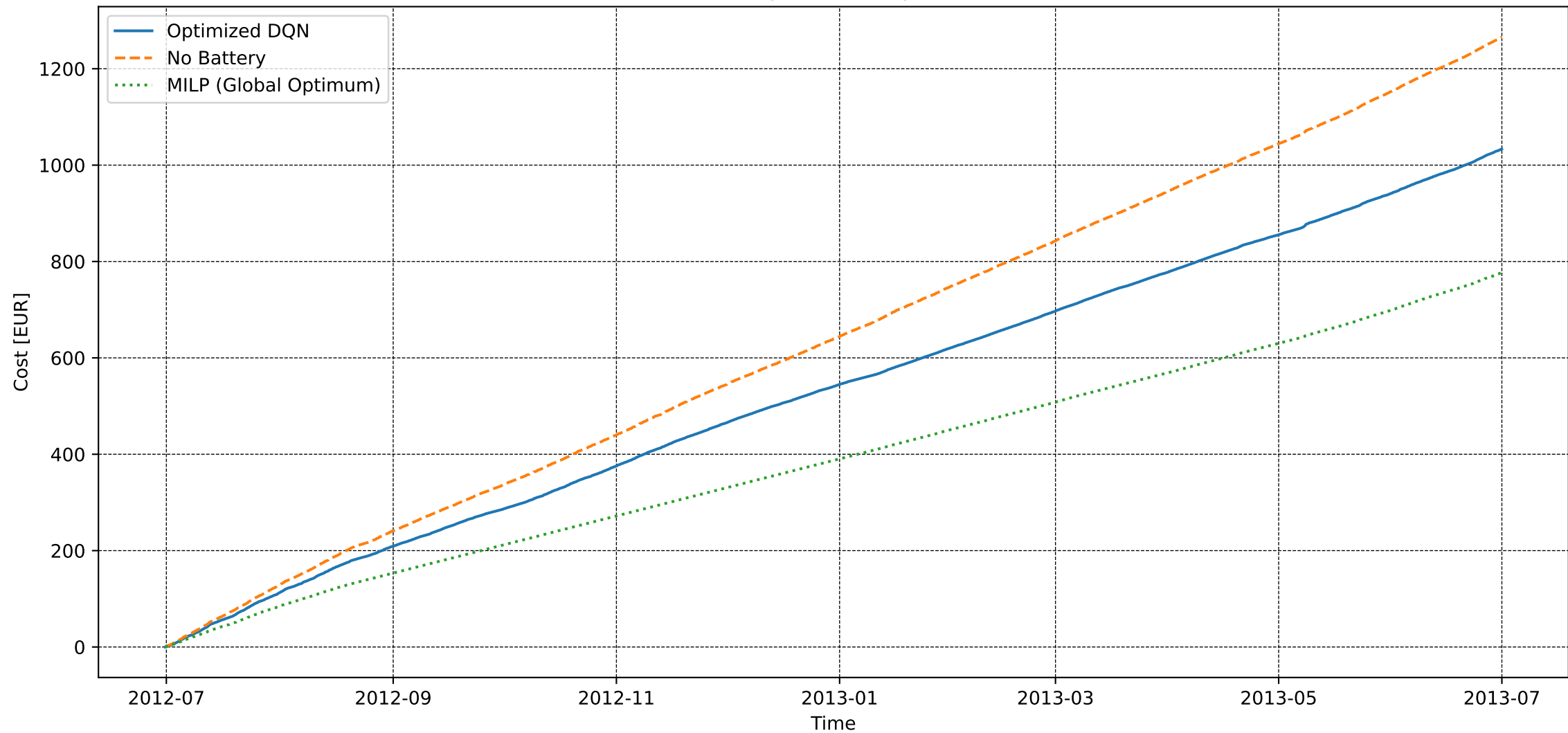
User 1 - Basic Training - Electricity Cost [DQN vs MILP]
